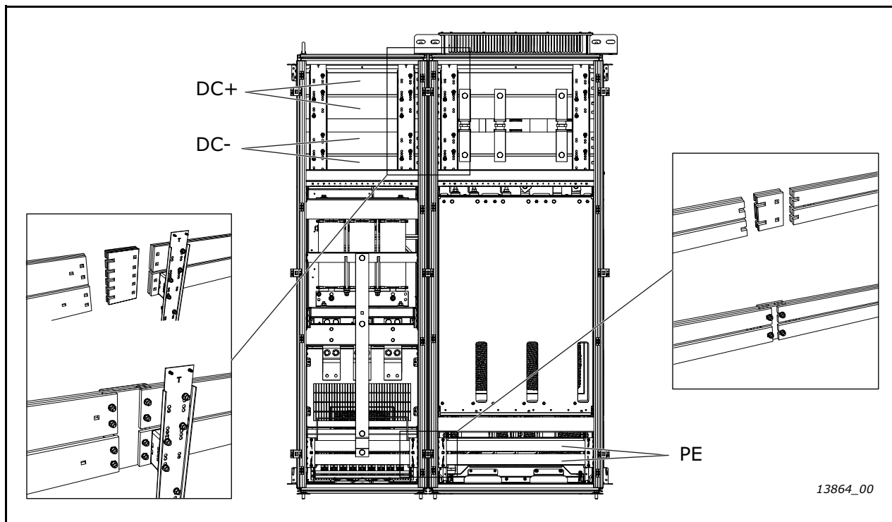
Figure 16. Connecting the common DC and PE busbars
