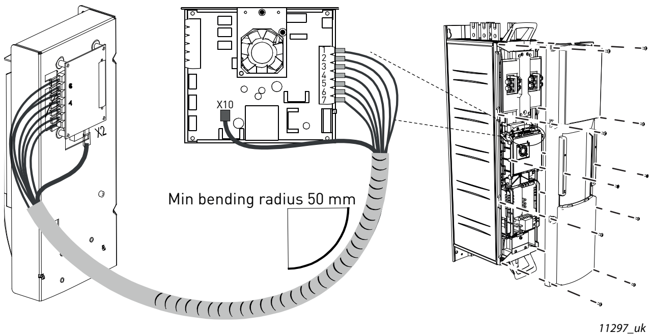
Figure 57. Connecting the power supply and control cables to the control unit, Ch7x
