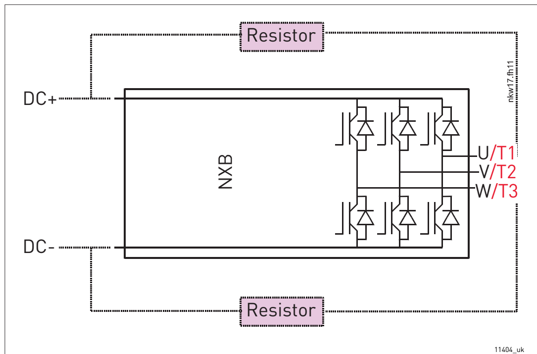
Figure 100. Vacon Brake Chopper Unit connections
