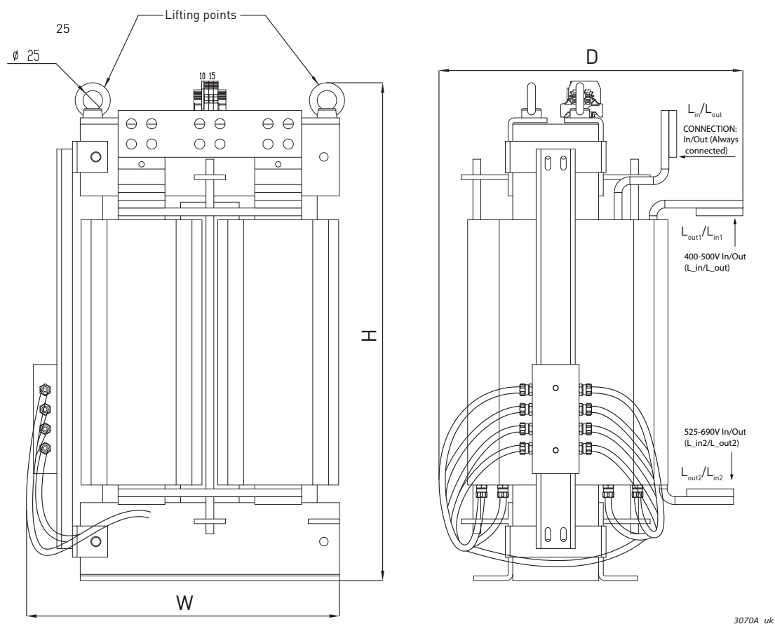
Figure 89. Example of L_{afe} choke of a Vacon RLC filter
