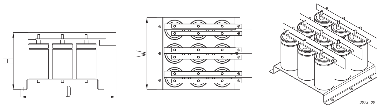
Figure 90. Example of capacitor bank ( C_{bank} ) of a Vacon RLC filter
