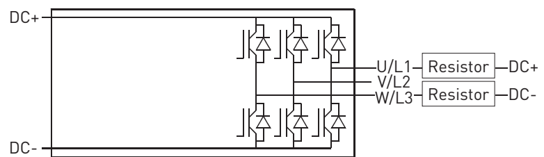
Figure 99. Brake chopper unit topology
