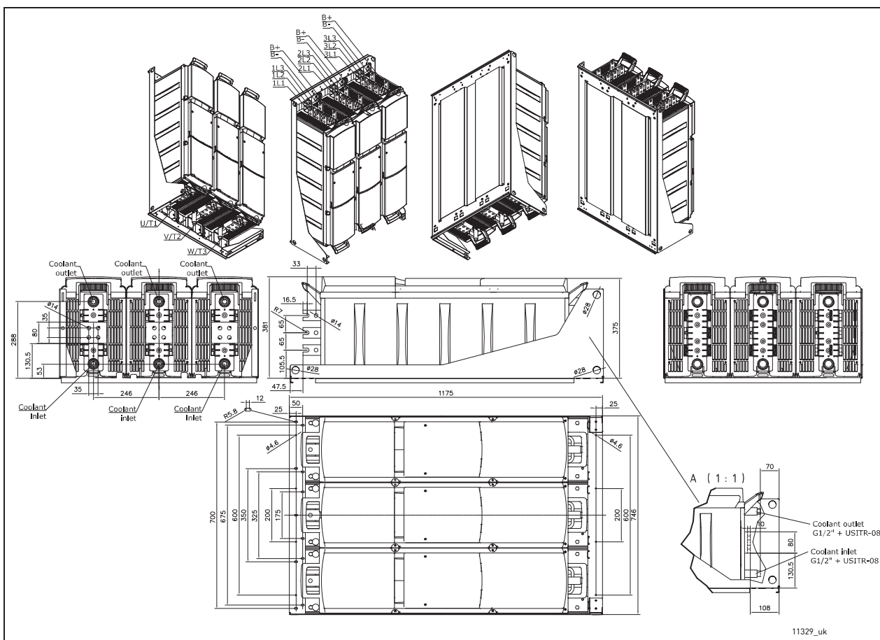
Figure 21. Vacon NX Liquid-Cooled frequency converter (6-pulse) dimensions, CH74, IP00
