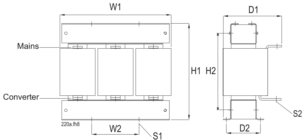
Figure 34. Example of input chokes for Vacon NX Liquid-Cooled. Sizes 87 A... 145 A and 590 A
