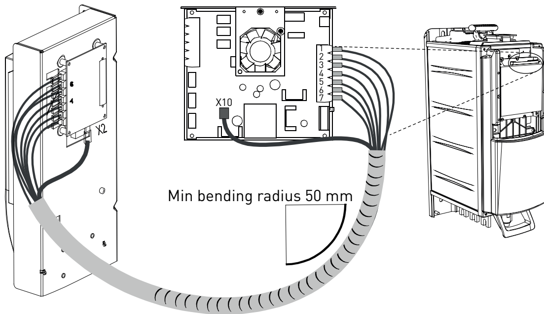
Figure 56. Connecting the power supply and control cables to the control unit, Ch6x
