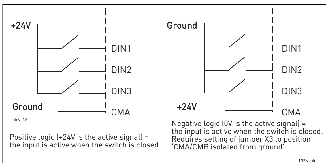
Figure 47. Positive/Negative logic
